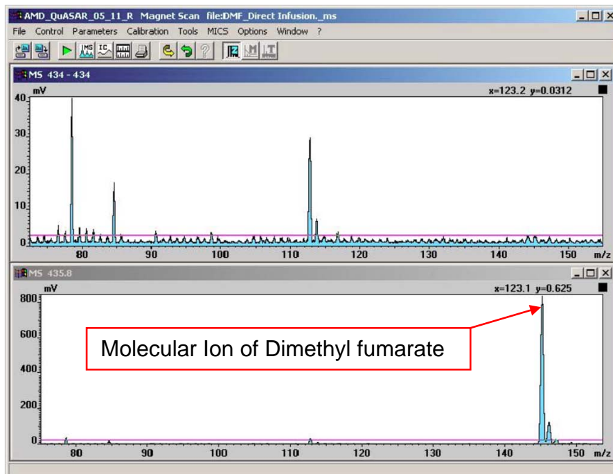
Fig. 1 Direct Sample Infusion of 100ng/μl DMF at 1 μL/min solvent flow; EI mass spectrum
