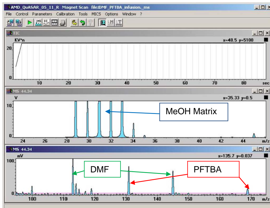
Fig. 2 Direct Sample Infusion of DMF/PFTBA including solvent matrix at 1 μl/min; EI mass spectrum incl. Reference Compound for Mass Determinations
